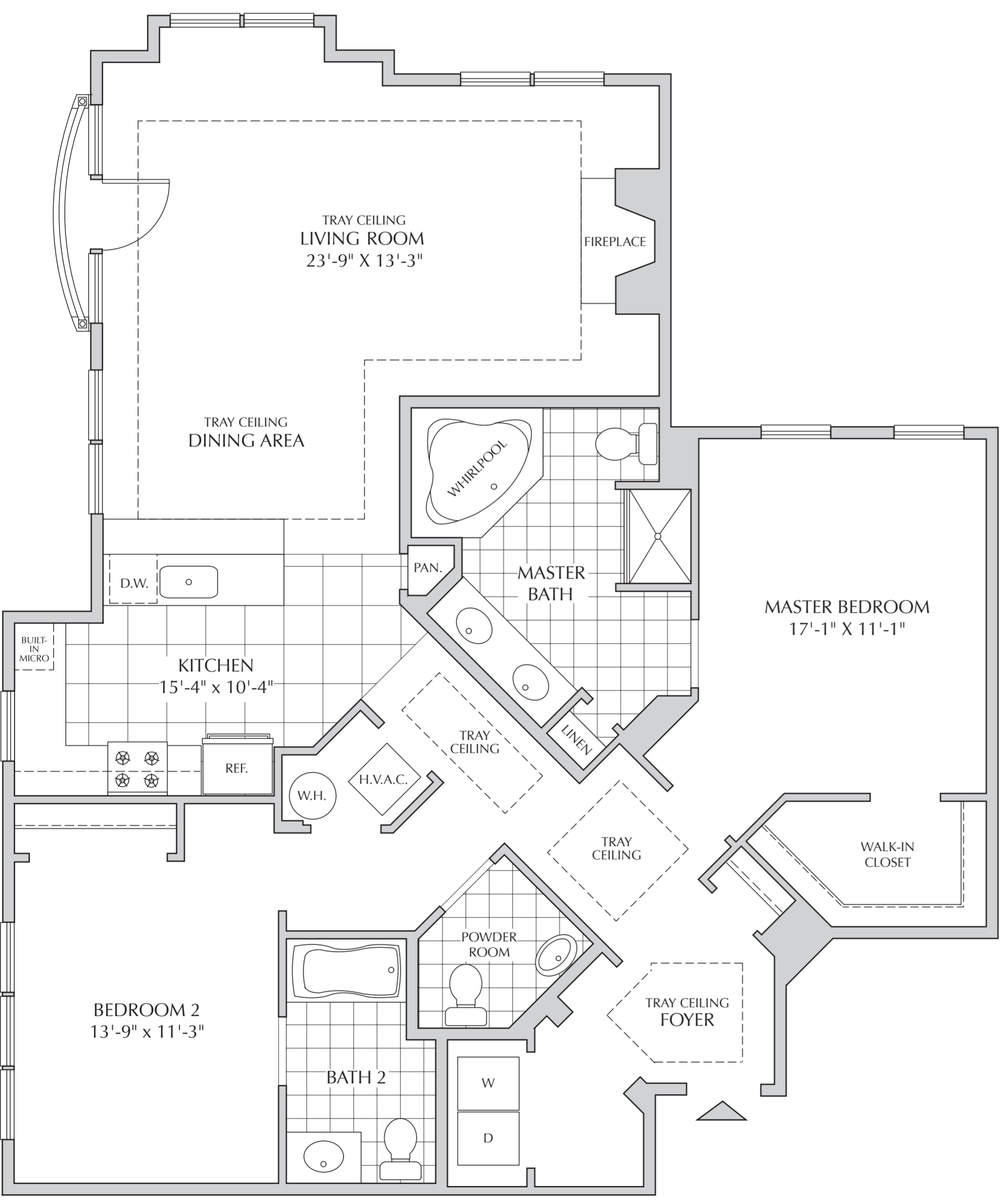
THE RESIDENCES AT PALMER SQUARE UU1
